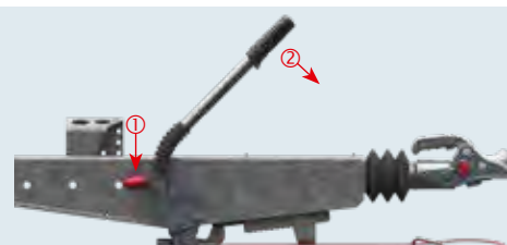
Handbrake lever applied = brake rod clamped
