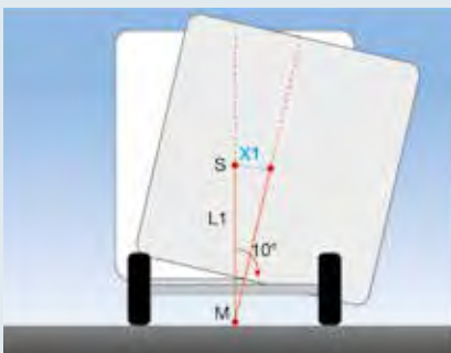
Conventional axle
