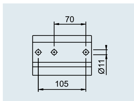
Jockey wheel flange
