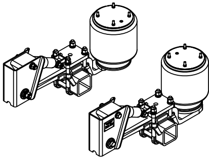
AUXILIARY VIEW
