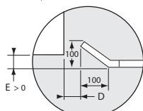
Detail 1 - Top view Detalle 1 - Vista superior
